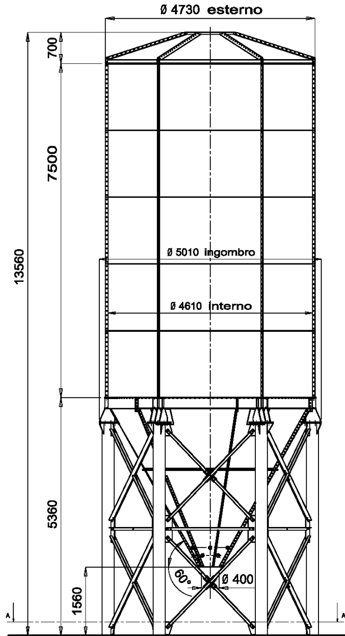
MODELLO CAMS 6CS5 CAPACITA' 150m 3
