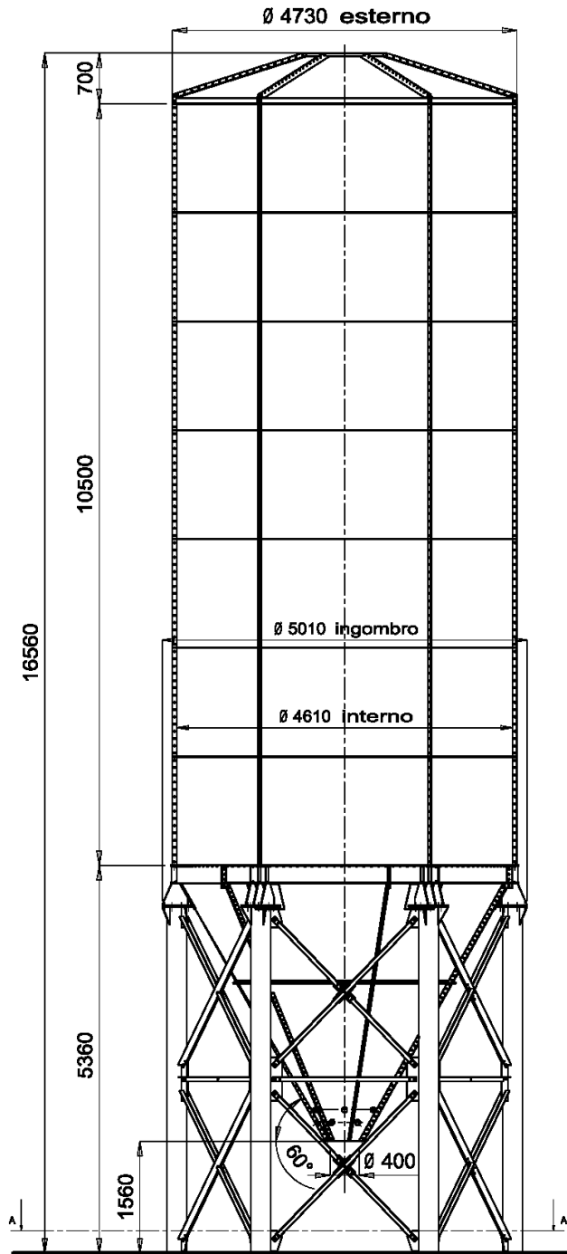
MODELLO CAMS 6CS7 CAPACITA' 200m 3
