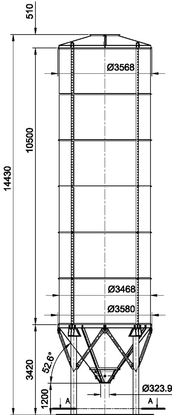
MODELLO CAMS CS105 105m 3
