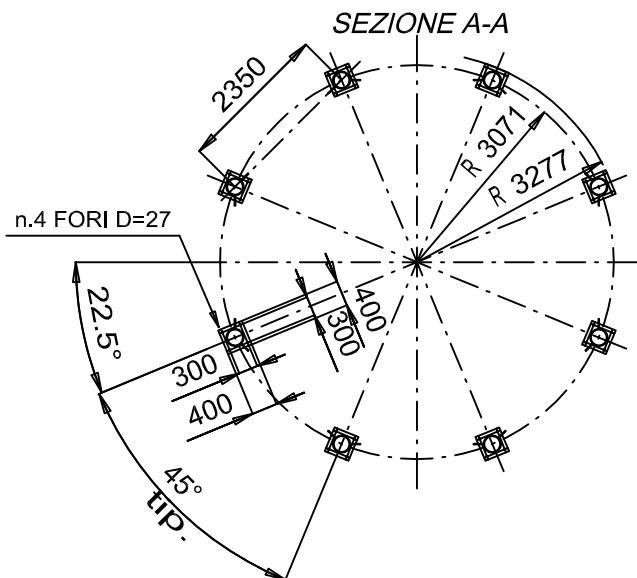
MODELLO CAMS 8CS8 CAPACITA' 410mc
