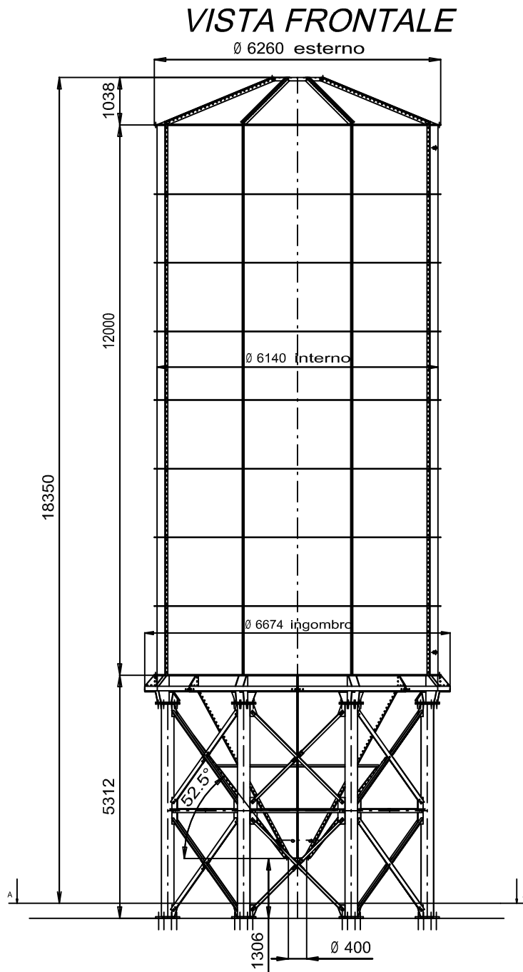
MODELLO CAMS 8CS8 CAPACITA' 410mc
